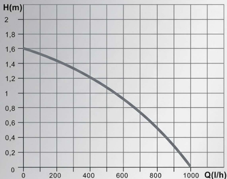
Dijagram protoka pumpi 1000
