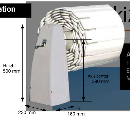
Electric box for 24V motor
